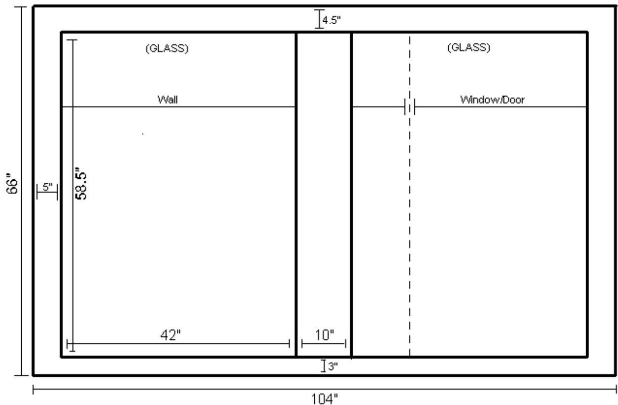
FRONTAL VIEW - FACING WINDOW FROM STREET
