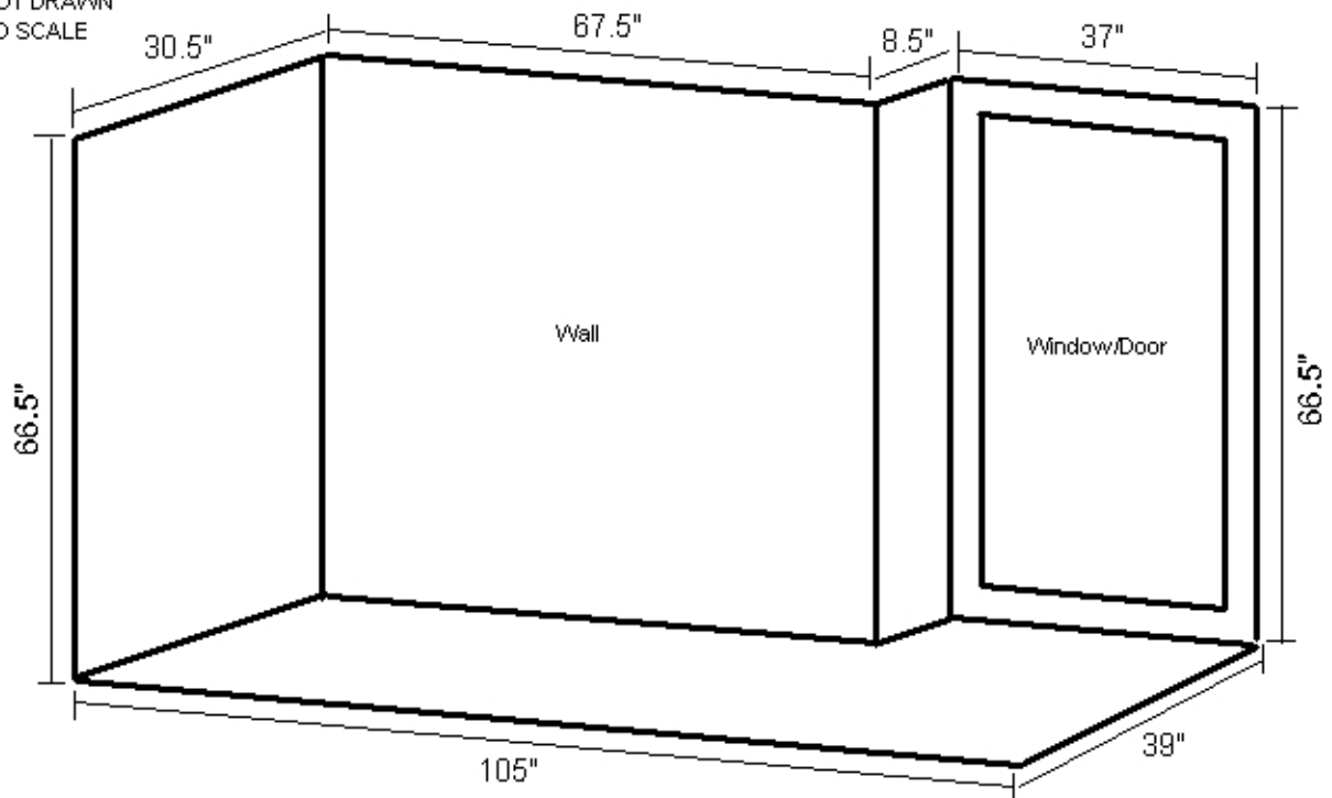
FRONTAL VIEW - FACING WINDOW FROM STREET
